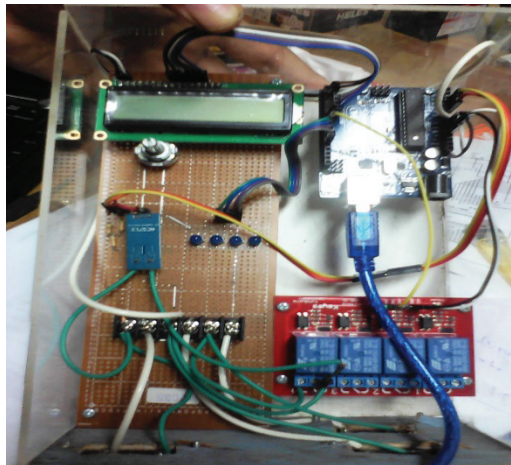
Figure 6. Assembled charging controller system
