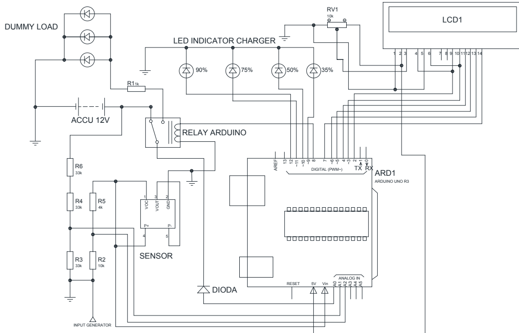
Figure 5. Controller system wiring diagram
