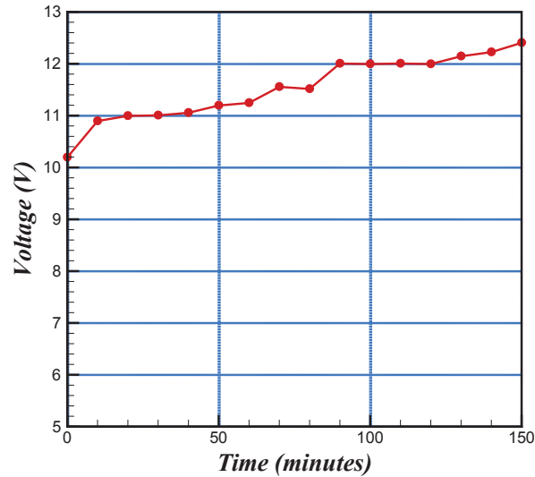
Figure 9. Charging time and process of 2 nd case
