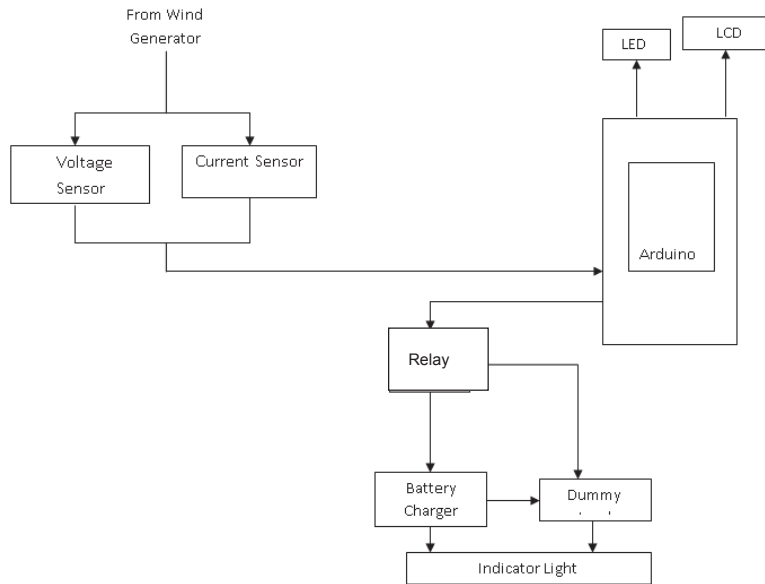
Figure 4. Charger components connection and workflow
