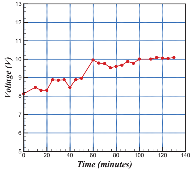
Figure 7. Charging time and voltage of 1 st case
